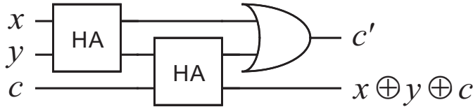
Figure 3.6. Full-adder circuit.
